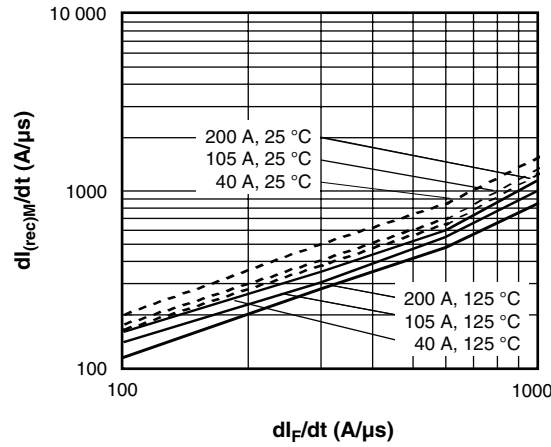
Fig. 8 - Typical dl_{(rec)M}/dt vs. di_F/dt (Per Leg)
